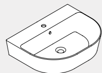
65x50xH16 cm FMLP06550TOM
